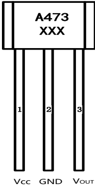
T092S
